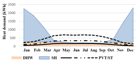
Figure 10 - Heat demand for a building in Amsterdam throughout the year for domestic heat water (DHW, orange) and space heating (SH, blue). The black lines are collectors with different areas [6].
