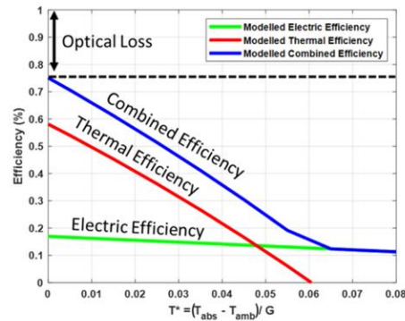
Figure 8 - Performance analysis of a PVT collector: highlighting electric efficiency (green), thermal efficiency (red), and combined efficiency (blue) [5].
