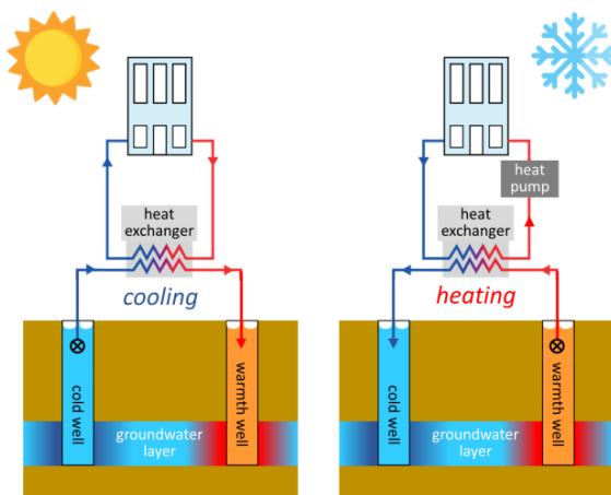
Figure 11 - Basic working principle of an ATEs system [7].
